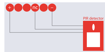
Normally Closed mode with PIR wiring diagram
