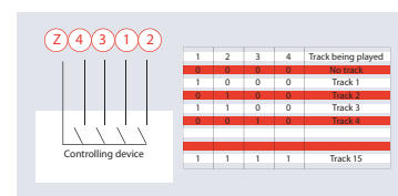
Binary controls for triggering
